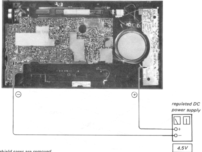
External 4.5V power-supply connection.
