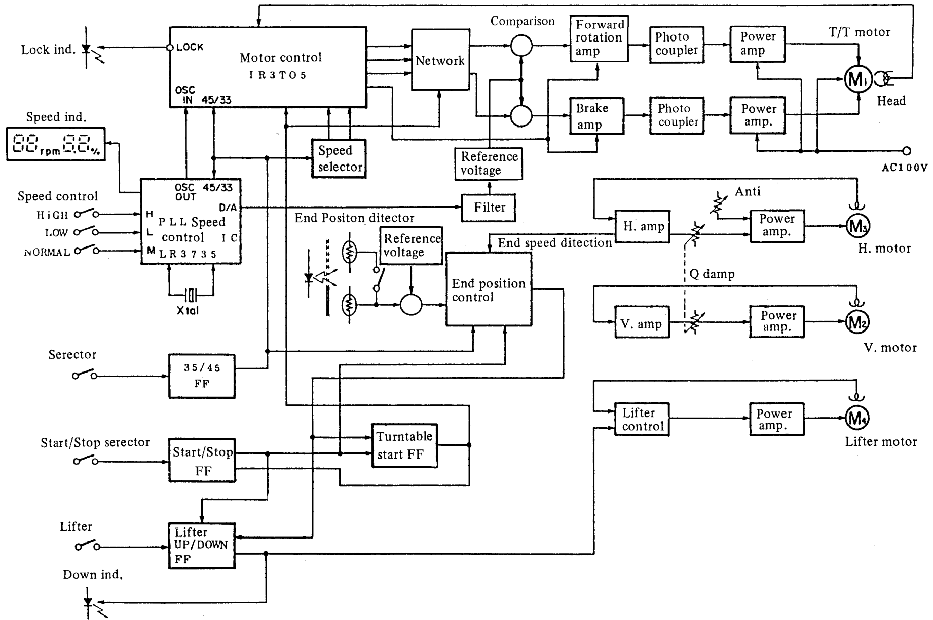
BLOCK DIAGRAM
