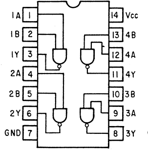
TC74HC00AP :PD74HC00P
