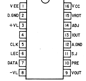
PCM61P
