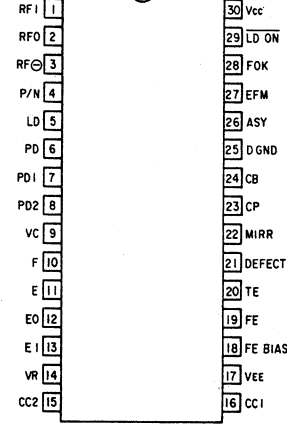
CXA1081S
