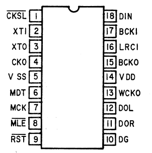
SM5840
