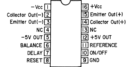
M5290P
