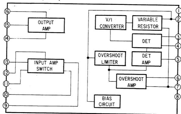
IC101, 104, 201, 204
