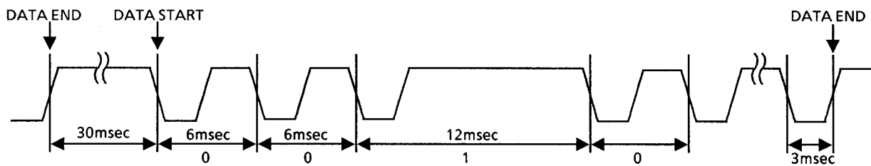
Input signal to RX-805VTN/VLTN
